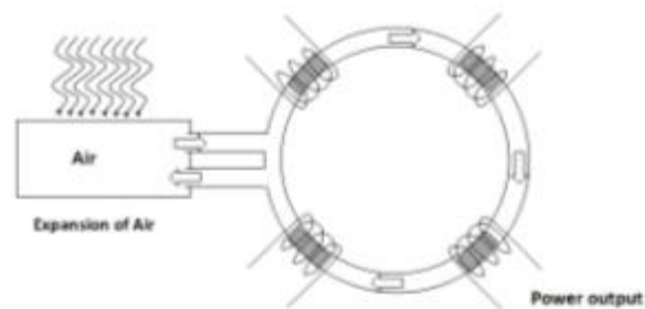
Solar Electric Power Generator using Ferrofluid - Concept
